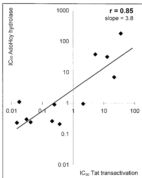
Fig. 2. Linear regression for IC_{50} values of NPA, c^3 NPA, DHCaA, c^3 DHCaA, C- c^3 Ado, 5'-noraristeromycin, KS606, NOM-14-6-1, NKO-6-16-3, (S)-DHPA, 6'-( R )-methyl-NPA, 6'-( R )-ethenyl-NPA, and 6'-( R )-ethynyl-NPA for their inhibition of AdoHcy hydrolase as a function of their IC_{50} values for Tat-transactivation of HIV-1.
