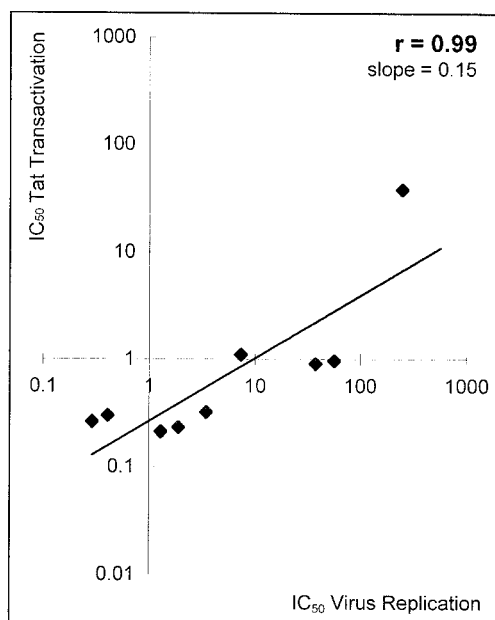
Fig. 3. Linear regression for IC_{50} values of NPA, c^3 NPA, DHCaA, c^3 DHCaA, C- c^3 Ado, (S)-DHPA, 6'-( R )-methyl-NPA, 6'-( R )-ethenyl-NPA, and 6'-( R )-ethynyl-NPA for their IC_{50} values of HIV-1 Tat-transactivation inhibition as function of their inhibition of HIV-1 replication in P4 cells.
