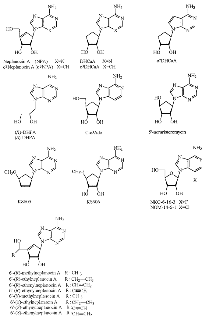
Fig. 1. Formulae of the adenosine analogues that were evaluated as inhibitors of AdoHcy hydrolase, HIV-1 replication, and Tat-transactivation.
