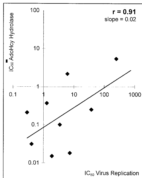
Fig. 4. Linear regression for IC_{50} values of NPA, c^3 NPA, DHCaA, c^3 DHCaA, C- c^3 Ado, (S)-DHPA, 6'-( R )-methyl-NPA, 6'-( R )-ethenyl-NPA, and 6'-( R )-ethynyl-NPA for their inhibition of HIV-1 replication in P4 cells as function of their IC_{50} values for AdoHcy hydrolase inhibition.
